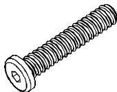
F: Bolt M6x45 (mm) Quantity: 4 pcs
