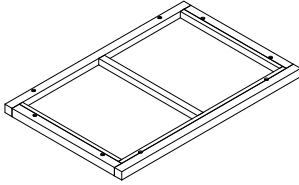
A: Top Frame 38x950x620 (mm) Quantity: 1 pc Box 3
